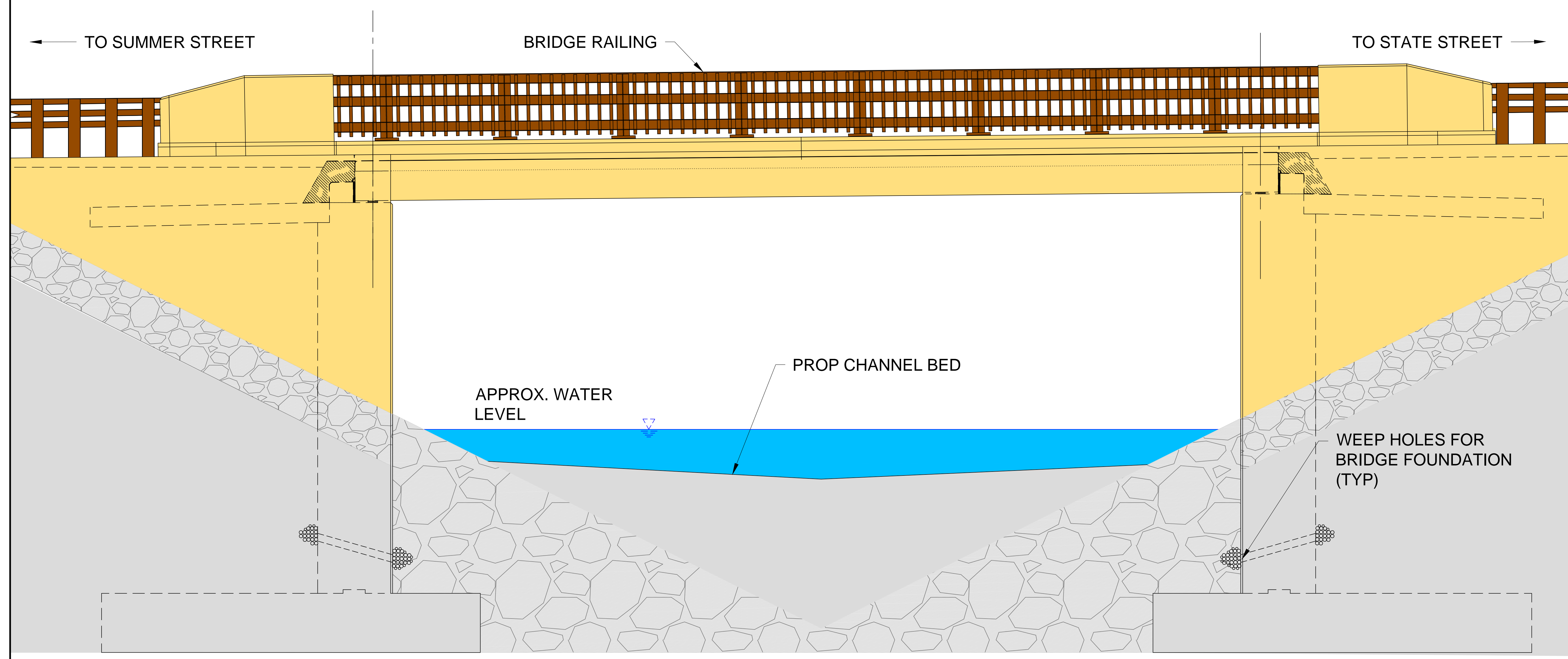
MILL STREET BRIDGE (LOOKING TOWARD PUFFER'S POND) SCALE: NONE
